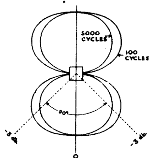
HORIZONTAL DIRECTIVITY OF VELOCITY MICROPHONE
