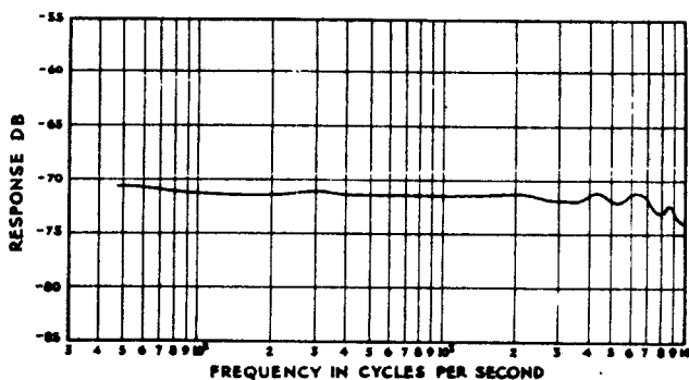
VELOCITY MICROPHONE FREQUENCY RESPONSE CURVE
